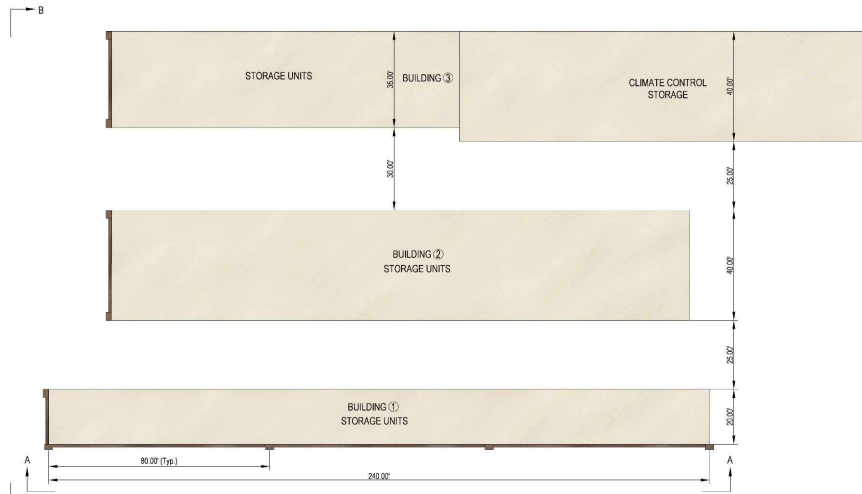
PLAN VIEW NOT TO SCALE
