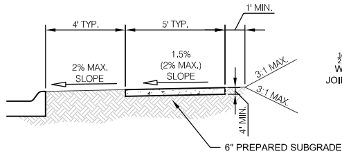
TYPICAL 4' OFFSET
