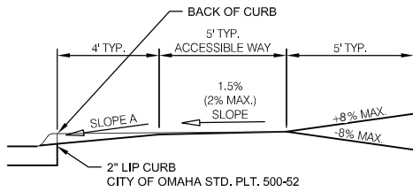
DRIVEWAY GRADES FOR 5' SIDEWALK W/4' SETBACK
