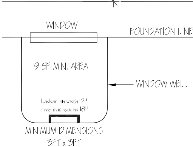
Section View NOT TO SCALE
